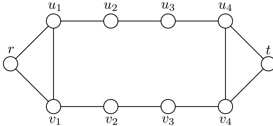
Figure 1: The graph G_4 .
