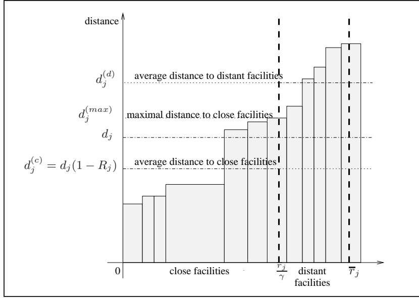
Fig. 1. Distances to facilities serving client j in \bar{x} . The width of a rectangle corresponding to facility i is equal to \bar{x}_{ij} . Figure helps to understand the meaning of R_j .
