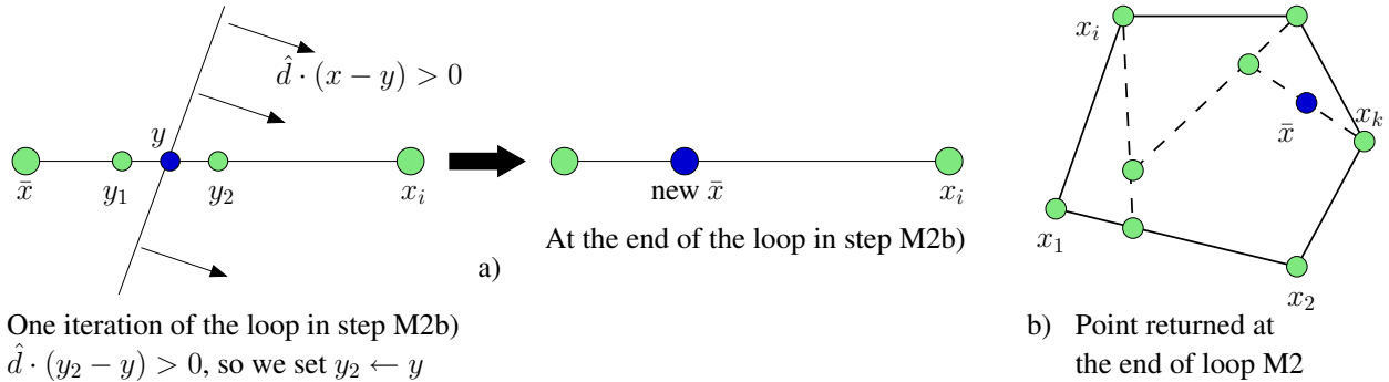
Figure 3: a) Binary search on one \bar{x} - x_i segment. b) Outcome of the iterative binary search procedure.
