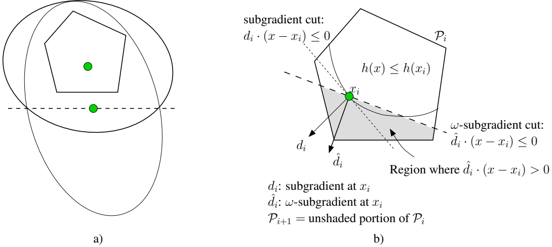
Figure 1: a) Cut derived from a violated inequality. b) Subgradient and \omega -subgradient cuts.
