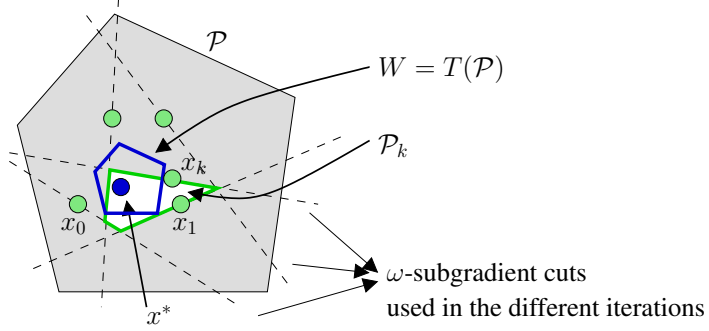
Figure 4: Pictorial description of the proof of Lemma 4.5
