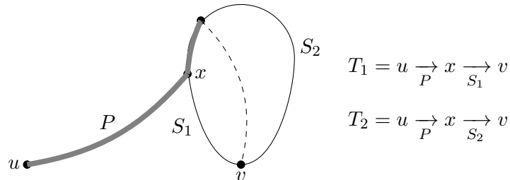
Figure 2: Path P makes its first contact with an odd (v, v) -trail.
