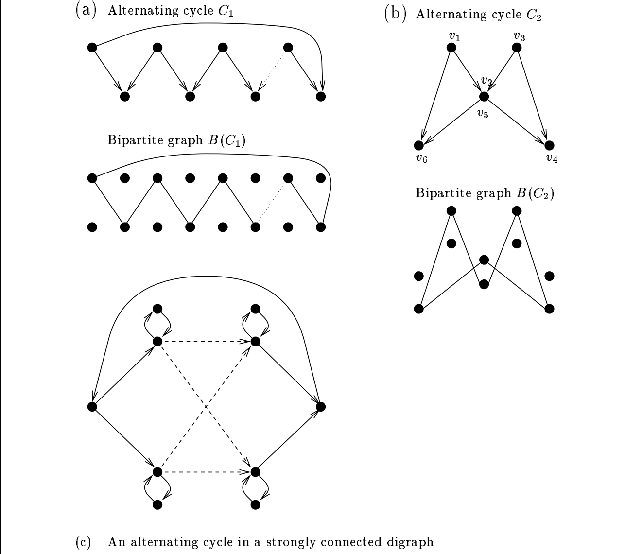
Figure 4: An illustration of an alternating cycle in a digraph, and of Mader’s theorem on critical alternating cycles in a k -node connected digraph, see Theorem 3.16.
