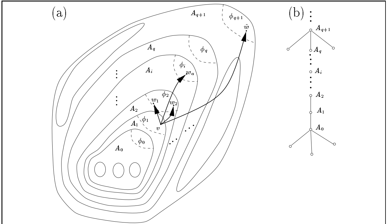
Figure 7: An illustration of Claim 2 in the proof of Theorem 4.8.
