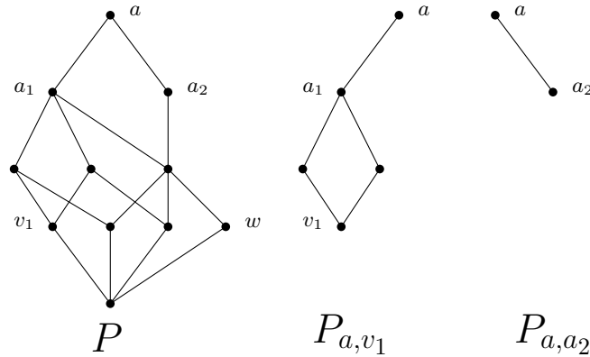
Figure 3.3: Lattice: P , P_{a,v_1} and P_{a,a_2}
