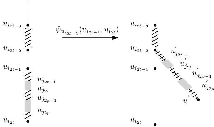
Figure 2.7: \tilde{\varphi}_{u_{i_{2l-2}}}(u_{i_{2l-1}}, u_{i_{2l}}) = u' and its corresponding sub-paths
