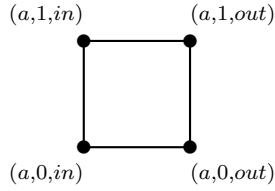
\langle V_a, E_a \rangle where a \in A
