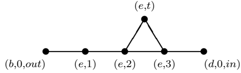
\langle V_e^0, E_e^0 \rangle where e = (b, d) \in R_0
