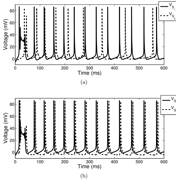
FIGURE 4: Cell 1 receives dendritic input I_{D_1} = 2.0 \mu A/cm^2 , cell 2 receives dendritic input I_{D_2} = 1.25 \mu A/cm^2 . (a) A weak AMPA connection: g_{AMPA_2} = 0.04 \text{ mS}/cm^2 . (b) A strong AMPA connection: g_{AMPA_2} = 0.2 \text{ mS}/cm^2 .
