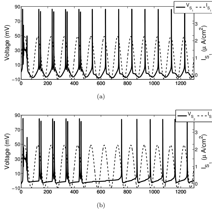
FIGURE 5: (a) The voltage of cell 1 and its corresponding input, I_{S_{cell1}}(t) . Note the synchronization to its input. (b) The voltage of cell 2 and the input from cell 1, I_{S_{cell1}}(t) . Cell 2 is synchronized to cell 1 until t = 500 ms, at which point it desynchronizes. At t = 500 ms the connection goes from strong to weak, and the applied sinusoidal current to cell 2 dominates.
