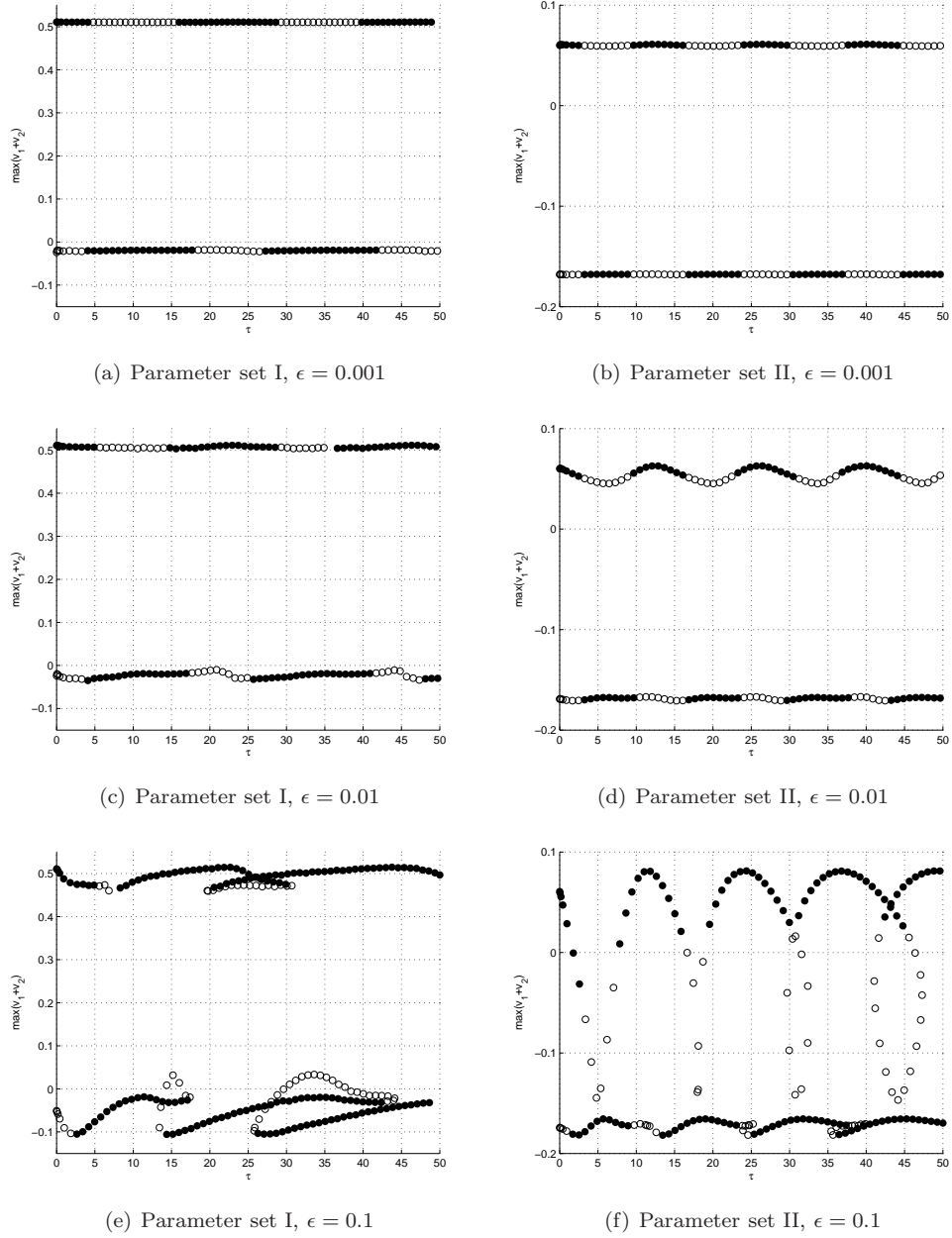
FIGURE 7. Results from numerical continuation study of in-phase and anti-phase periodic solutions in the Morris-Lecar model (22) with parameter values as given in Table 1 and \epsilon as shown. The amplitude of the periodic solutions (represented as \max(v_1(t) + v_2(t)) , 0 \leq t \leq T ) is plotted vs the time delay, \tau . In all cases, the upper curve corresponds to the in-phase solution and the lower curve and the anti-phase solution. Filled/open circles denote stable/unstable solutions.
